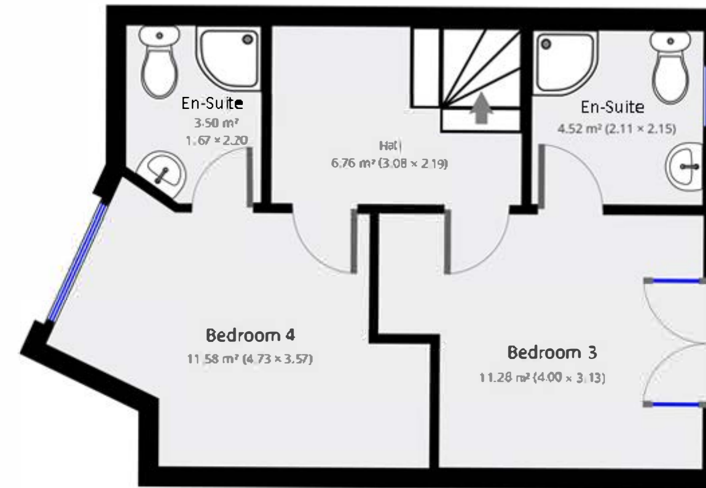
2nd Floor
