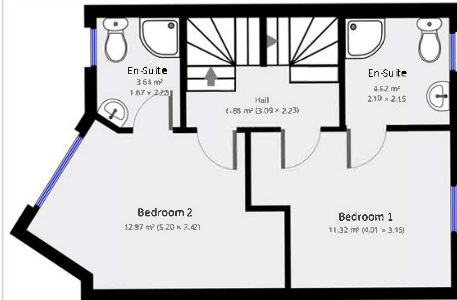
1st Floor
