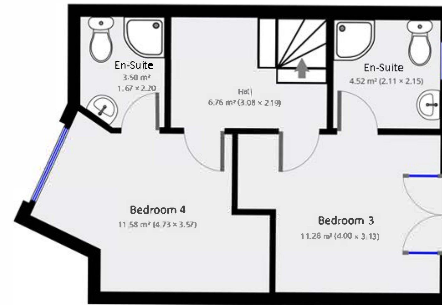
2nd Floor
